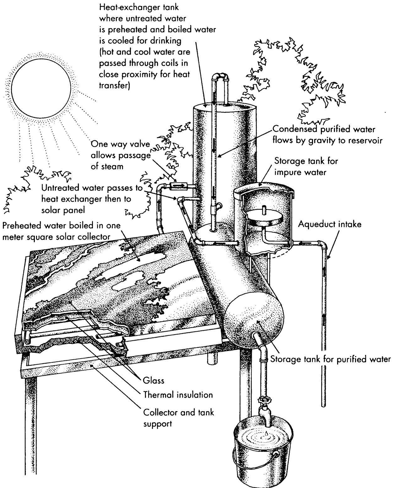
The Gaviotas Solar Kettle for Sterilizing Water
